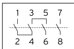
4 Pole with jumper link
