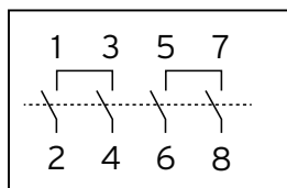
2 Pole in series & 2 Pole in parallel
